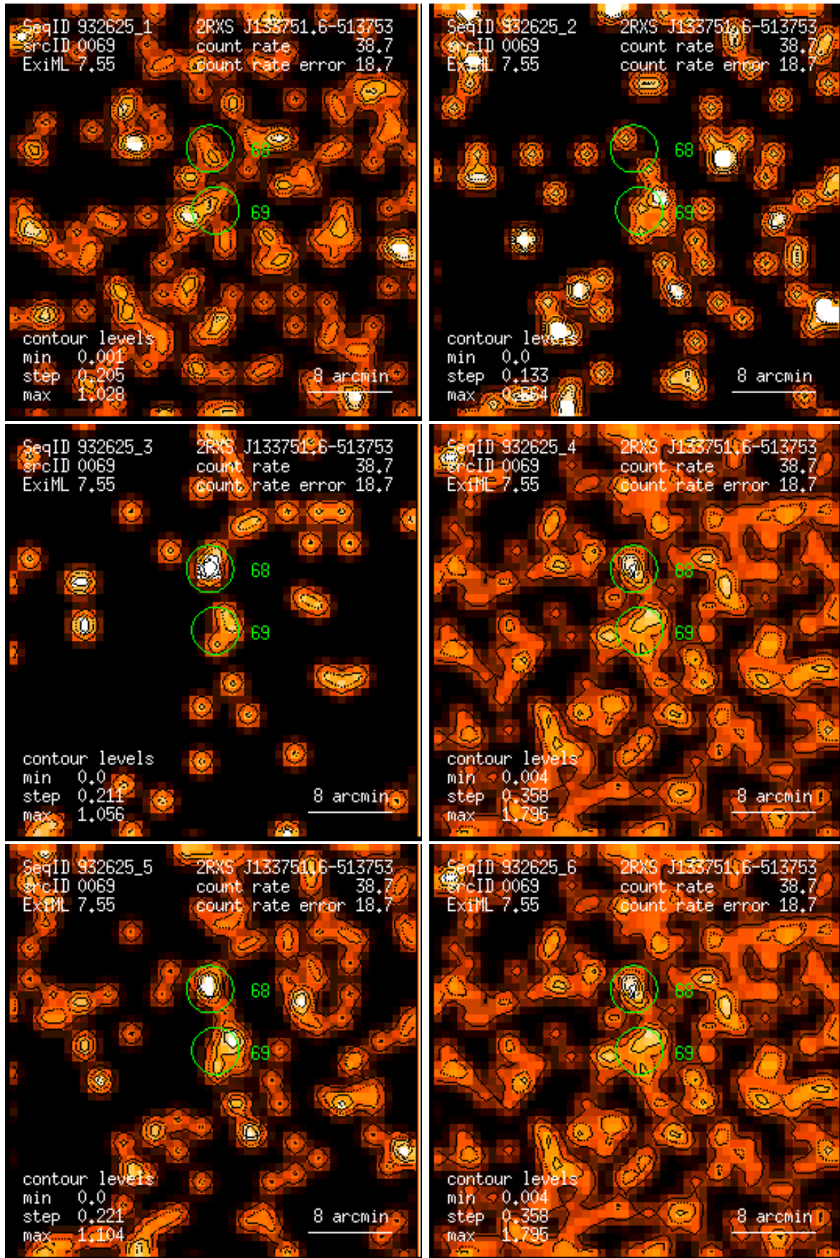
Figure 69: RASS 932625: detection 0069: band rate images, Gaussian filter: (1) PSPC channels 11 – 41, (2) 52 – 90, (3) 91 – 201, (4) 11 – 235, (5) 52 – 201, (6) 11 – 201. Broad band rates in counts/ks. Band rate contour levels in counts/ks/arcmin 2 .
