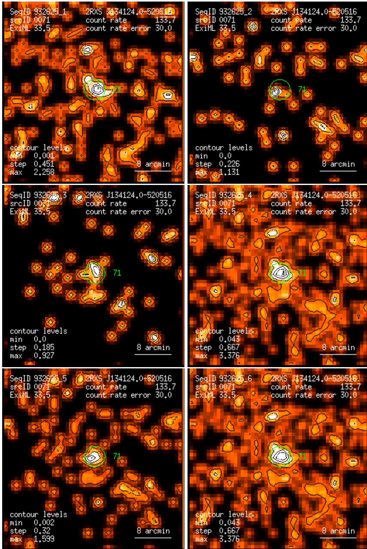
Figure 71: RASS 932625: detection 0071: band rate images, Gaussian filter: (1) PSPC channels 11 – 41, (2) 52 – 90, (3) 91 – 201, (4) 11 – 235, (5) 52 – 201, (6) 11 – 201. Broad band rates in counts/ks. Band rate contour levels in counts/ks/arcmin 2 .
