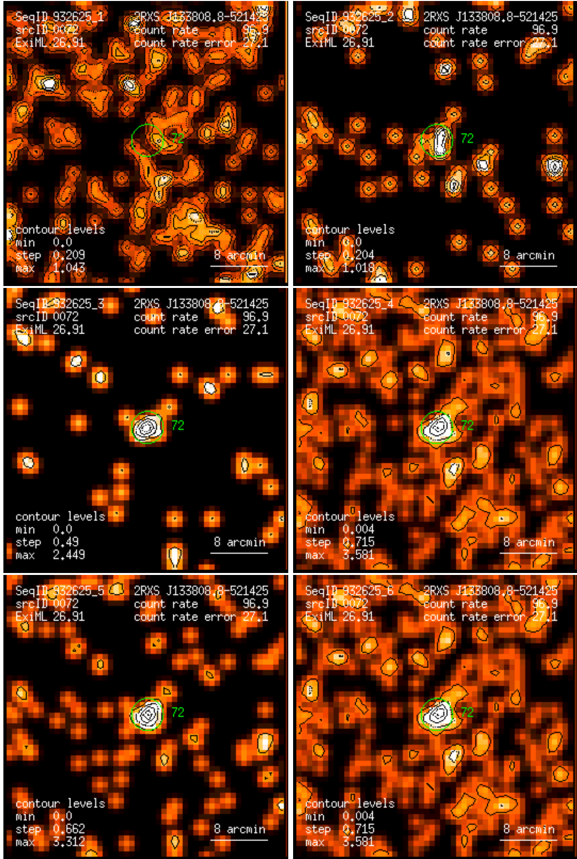
Figure 72: RASS 932625: detection 0072: band rate images, Gaussian filter: (1) PSPC channels 11 – 41, (2) 52 – 90, (3) 91 – 201, (4) 11 – 235, (5) 52 – 201, (6) 11 – 201. Broad band rates in counts/ks. Band rate contour levels in counts/ks/arcmin 2 .
