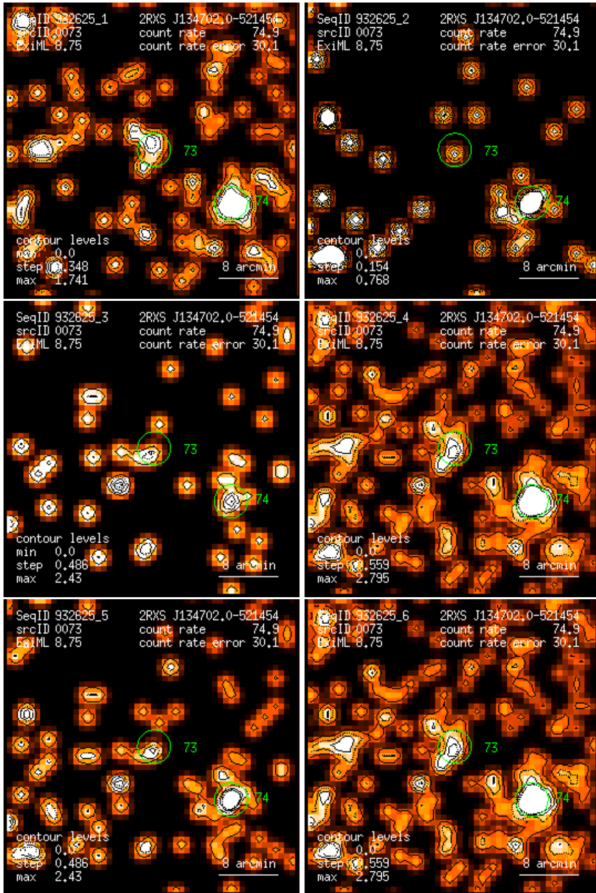
Figure 73: RASS 932625: detection 0073: band rate images, Gaussian filter: (1) PSPC channels 11 – 41, (2) 52 – 90, (3) 91 – 201, (4) 11 – 235, (5) 52 – 201, (6) 11 – 201. Broad band rates in counts/ks. Band rate contour levels in counts/ks/arcmin 2 .
