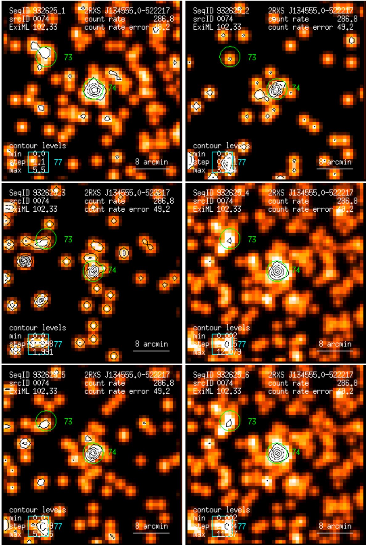
Figure 74: RASS 932625: detection 0074: band rate images, Gaussian filter: (1) PSPC channels 11 – 41, (2) 52 – 90, (3) 91 – 201, (4) 11 – 235, (5) 52 – 201, (6) 11 – 201. Broad band rates in counts/ks. Band rate contour levels in counts/ks/arcmin 2 .
