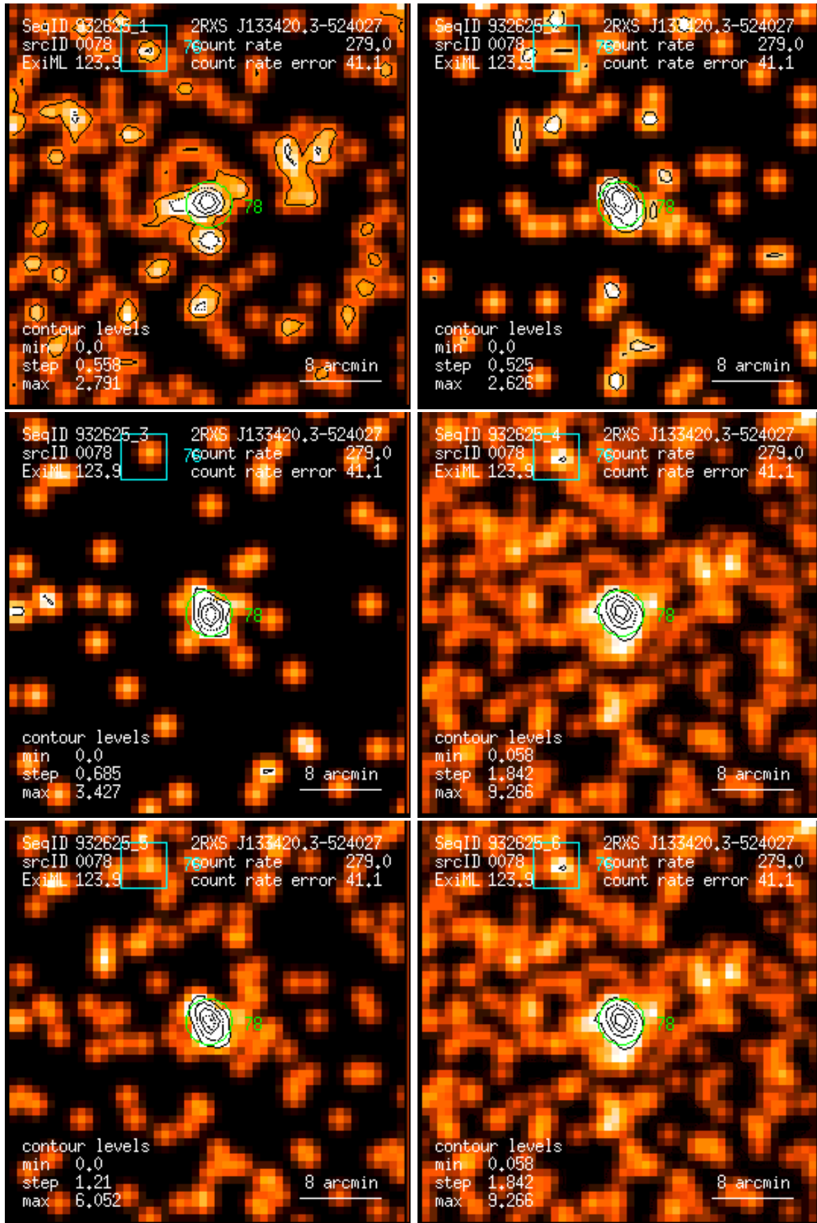
Figure 78: RASS 932625: detection 0078: band rate images, Gaussian filter: (1) PSPC channels 11 – 41, (2) 52 – 90, (3) 91 – 201, (4) 11 – 235, (5) 52 – 201, (6) 11 – 201. Broad band rates in counts/ks. Band rate contour levels in counts/ks/arcmin 2 .
