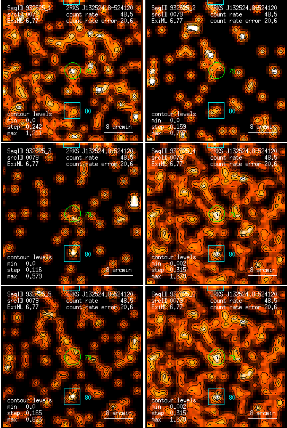
Figure 79: RASS 932625: detection 0079: band rate images, Gaussian filter: (1) PSPC channels 11 – 41, (2) 52 – 90, (3) 91 – 201, (4) 11 – 235, (5) 52 – 201, (6) 11 – 201. Broad band rates in counts/ks. Band rate contour levels in counts/ks/arcmin 2 .
