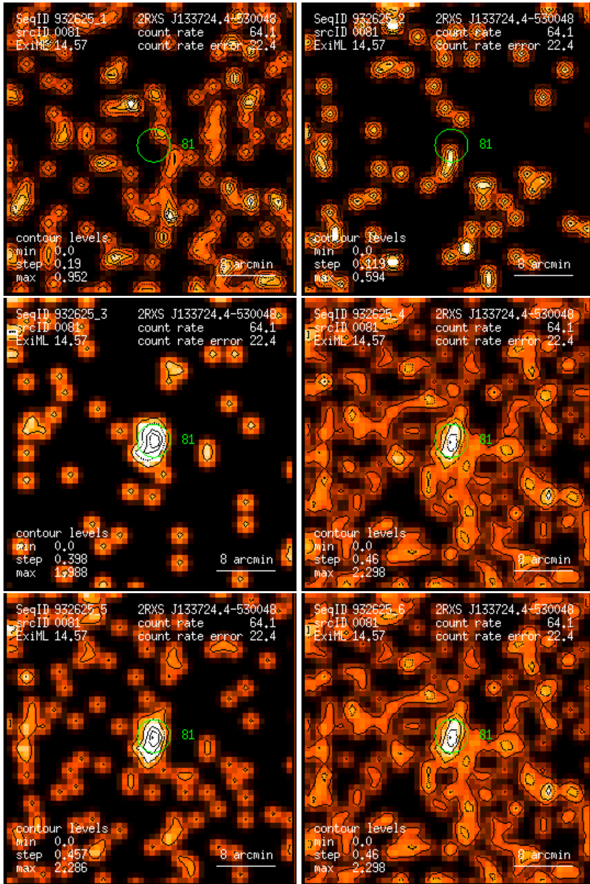
Figure 81: RASS 932625: detection 0081: band rate images, Gaussian filter: (1) PSPC channels 11 – 41, (2) 52 – 90, (3) 91 – 201, (4) 11 – 235, (5) 52 – 201, (6) 11 – 201. Broad band rates in counts/ks. Band rate contour levels in counts/ks/arcmin 2 .
