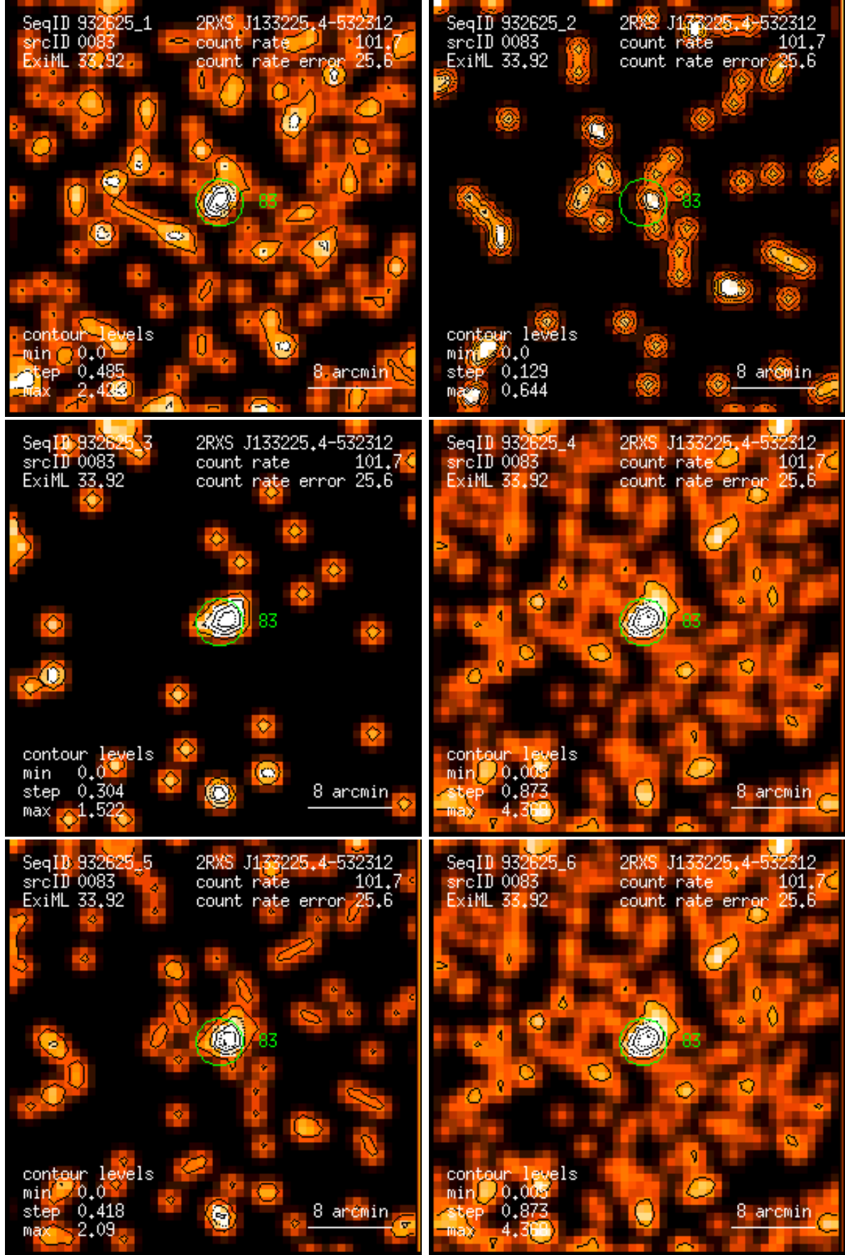
Figure 83: RASS 932625: detection 0083: band rate images, Gaussian filter: (1) PSPC channels 11 – 41, (2) 52 – 90, (3) 91 – 201, (4) 11 – 235, (5) 52 – 201, (6) 11 – 201. Broad band rates in counts/ks. Band rate contour levels in counts/ks/arcmin 2 .
