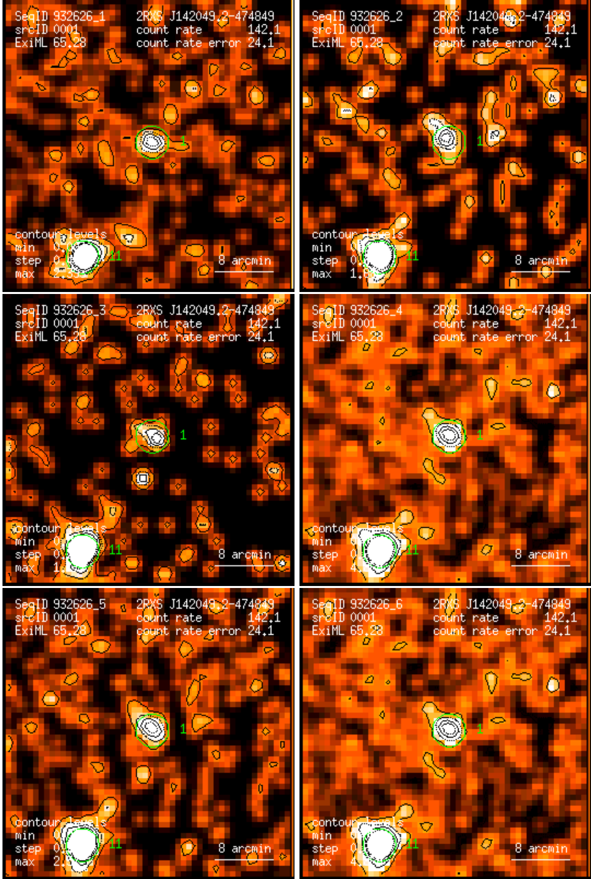
Figure 1: RASS 932626: detection 0001: band rate images, Gaussian filter: (1) PSPC channels 11 – 41, (2) 52 – 90, (3) 91 – 201, (4) 11 – 235, (5) 52 – 201, (6) 11 – 201. Broad band rates in counts/ks. Band rate contour levels in counts/ks/arcmin 2 .
