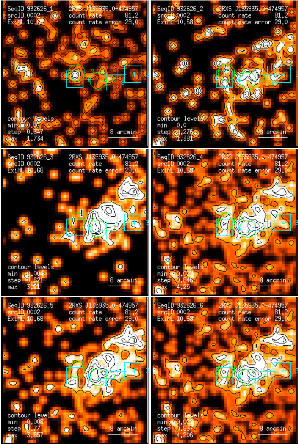
Figure 2: RASS 932626: detection 0002: band rate images, Gaussian filter: (1) PSPC channels 11 – 41, (2) 52 – 90, (3) 91 – 201, (4) 11 – 235, (5) 52 – 201, (6) 11 – 201. Broad band rates in counts/ks. Band rate contour levels in counts/ks/arcmin 2 .
