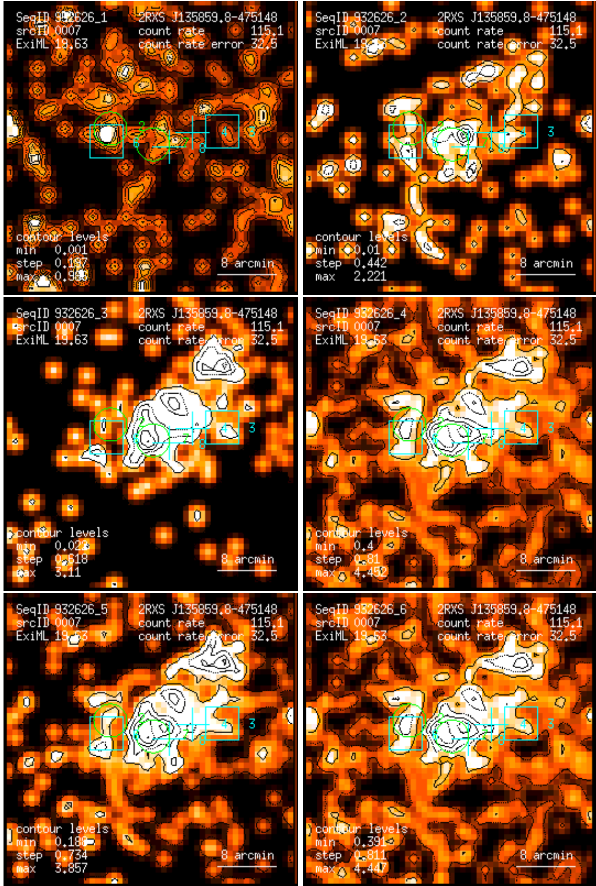
Figure 7: RASS 932626: detection 0007: band rate images, Gaussian filter: (1) PSPC channels 11 – 41, (2) 52 – 90, (3) 91 – 201, (4) 11 – 235, (5) 52 – 201, (6) 11 – 201. Broad band rates in counts/ks. Band rate contour levels in counts/ks/arcmin 2 .
