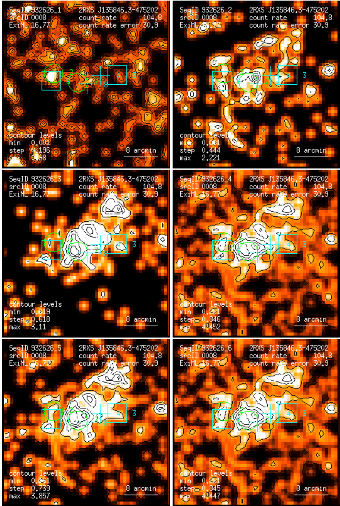
Figure 8: RASS 932626: detection 0008: band rate images, Gaussian filter: (1) PSPC channels 11 – 41, (2) 52 – 90, (3) 91 – 201, (4) 11 – 235, (5) 52 – 201, (6) 11 – 201. Broad band rates in counts/ks. Band rate contour levels in counts/ks/arcmin 2 .
