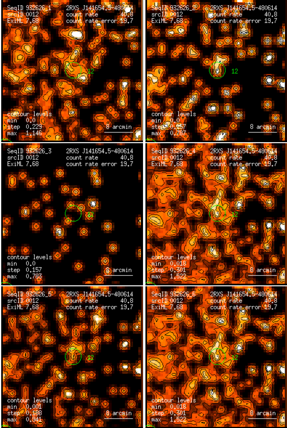
Figure 12: RASS 932626: detection 0012: band rate images, Gaussian filter: (1) PSPC channels 11 – 41, (2) 52 – 90, (3) 91 – 201, (4) 11 – 235, (5) 52 – 201, (6) 11 – 201. Broad band rates in counts/ks. Band rate contour levels in counts/ks/arcmin 2 .
