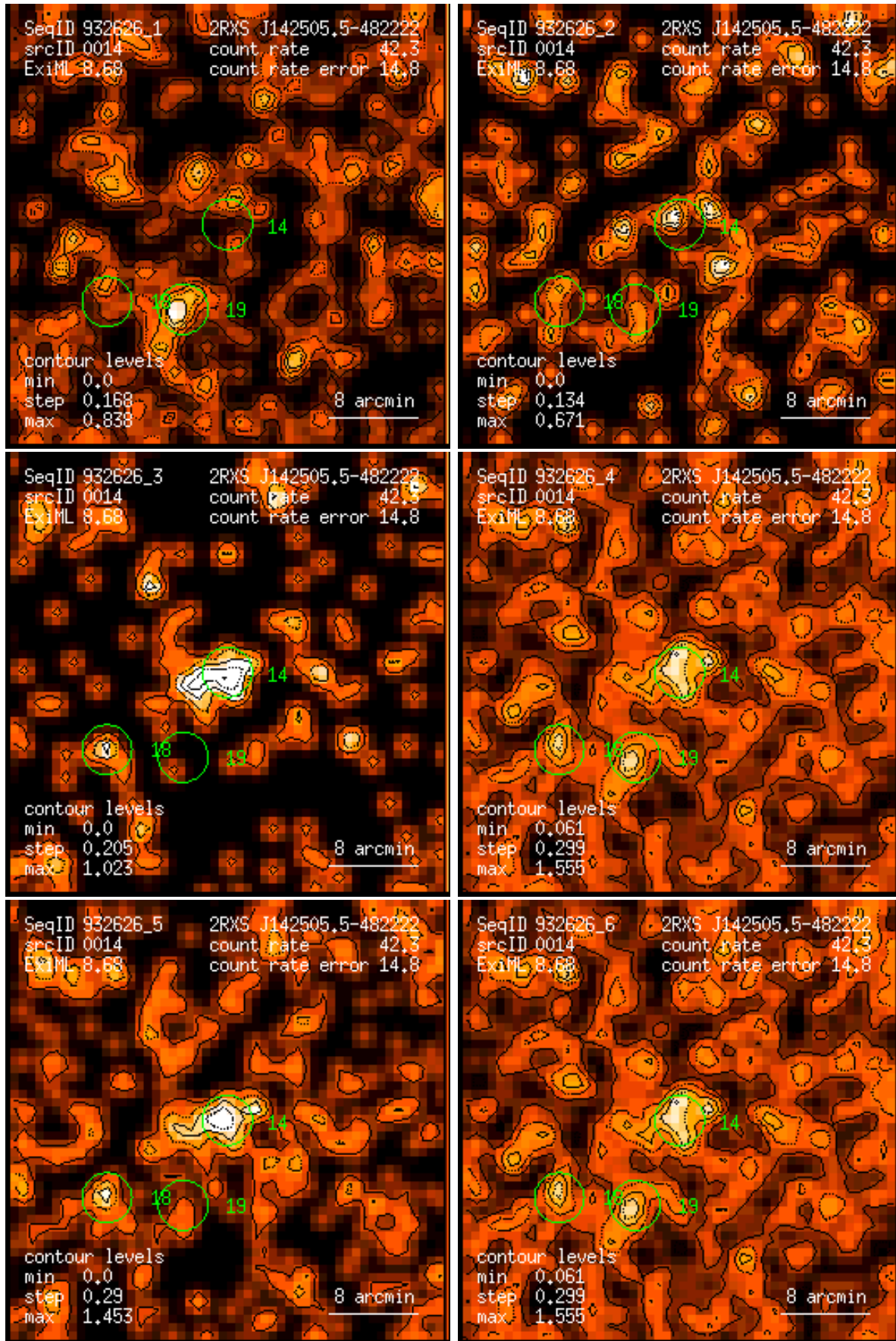
Figure 14: RASS 932626: detection 0014: band rate images, Gaussian filter: (1) PSPC channels 11 – 41, (2) 52 – 90, (3) 91 – 201, (4) 11 – 235, (5) 52 – 201, (6) 11 – 201. Broad band rates in counts/ks. Band rate contour levels in counts/ks/arcmin 2 .
