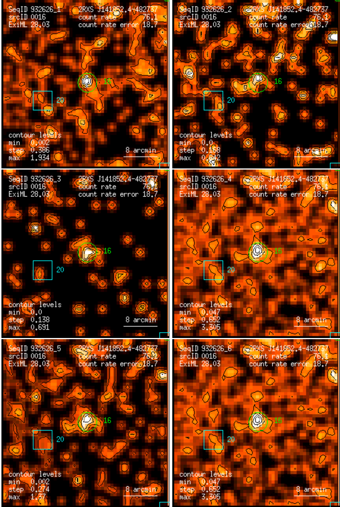
Figure 16: RASS 932626: detection 0016: band rate images, Gaussian filter: (1) PSPC channels 11 – 41, (2) 52 – 90, (3) 91 – 201, (4) 11 – 235, (5) 52 – 201, (6) 11 – 201. Broad band rates in counts/ks. Band rate contour levels in counts/ks/arcmin 2 .
