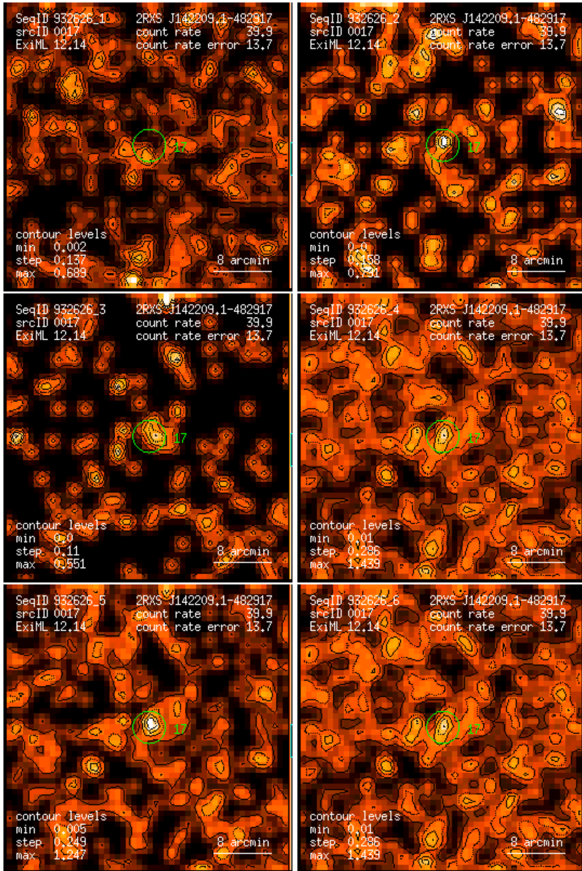
Figure 17: RASS 932626: detection 0017: band rate images, Gaussian filter: (1) PSPC channels 11 – 41, (2) 52 – 90, (3) 91 – 201, (4) 11 – 235, (5) 52 – 201, (6) 11 – 201. Broad band rates in counts/ks. Band rate contour levels in counts/ks/arcmin 2 .
