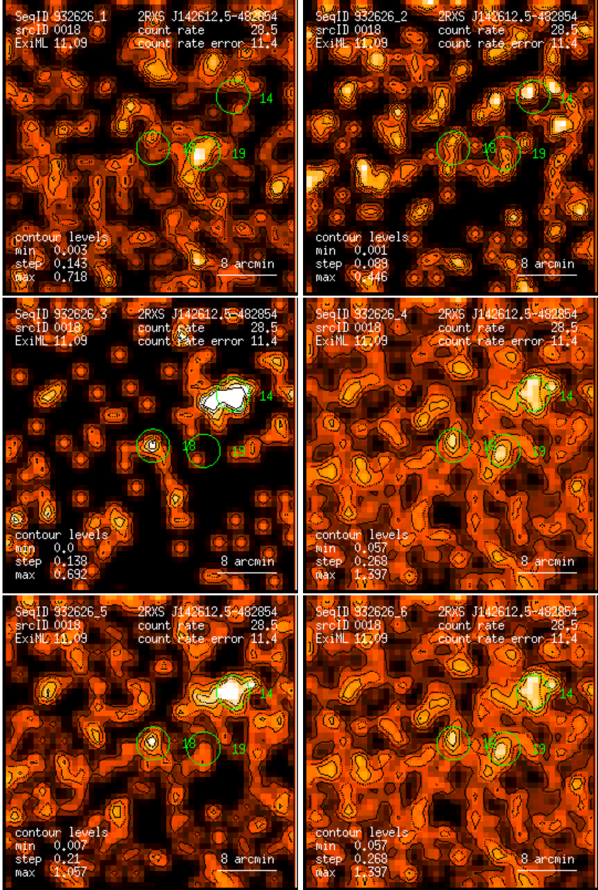
Figure 18: RASS 932626: detection 0018: band rate images, Gaussian filter: (1) PSPC channels 11 – 41, (2) 52 – 90, (3) 91 – 201, (4) 11 – 235, (5) 52 – 201, (6) 11 – 201. Broad band rates in counts/ks. Band rate contour levels in counts/ks/arcmin 2 .
