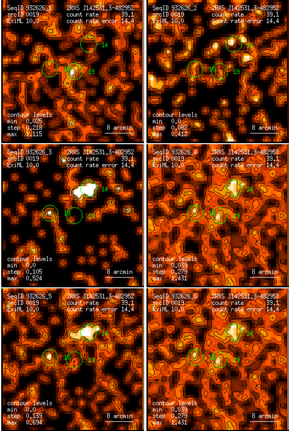
Figure 19: RASS 932626: detection 0019: band rate images, Gaussian filter: (1) PSPC channels 11 – 41, (2) 52 – 90, (3) 91 – 201, (4) 11 – 235, (5) 52 – 201, (6) 11 – 201. Broad band rates in counts/ks. Band rate contour levels in counts/ks/arcmin 2 .
