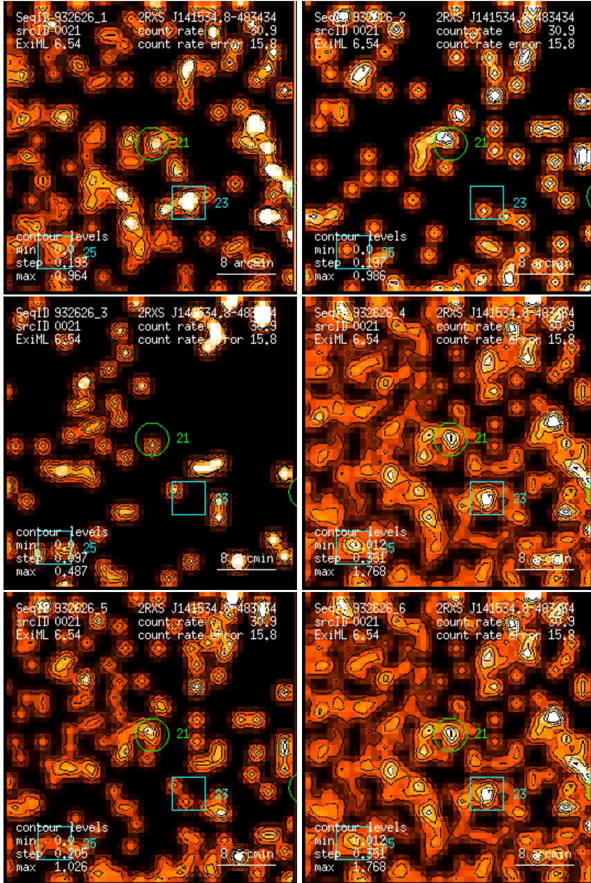
Figure 21: RASS 932626: detection 0021: band rate images, Gaussian filter: (1) PSPC channels 11 – 41, (2) 52 – 90, (3) 91 – 201, (4) 11 – 235, (5) 52 – 201, (6) 11 – 201. Broad band rates in counts/ks. Band rate contour levels in counts/ks/arcmin 2 .
