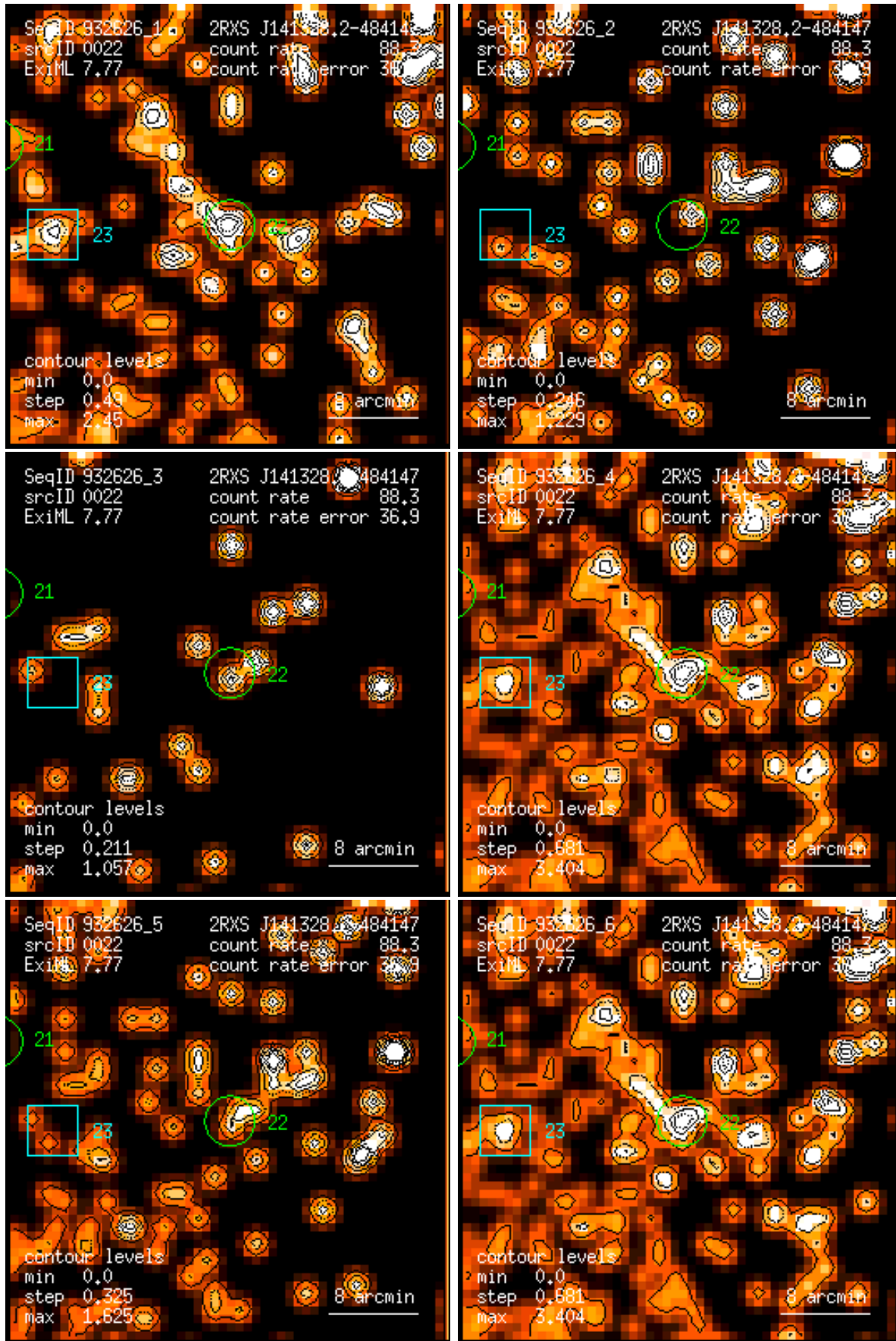
Figure 22: RASS 932626: detection 0022: band rate images, Gaussian filter: (1) PSPC channels 11 – 41, (2) 52 – 90, (3) 91 – 201, (4) 11 – 235, (5) 52 – 201, (6) 11 – 201. Broad band rates in counts/ks. Band rate contour levels in counts/ks/arcmin 2 .
