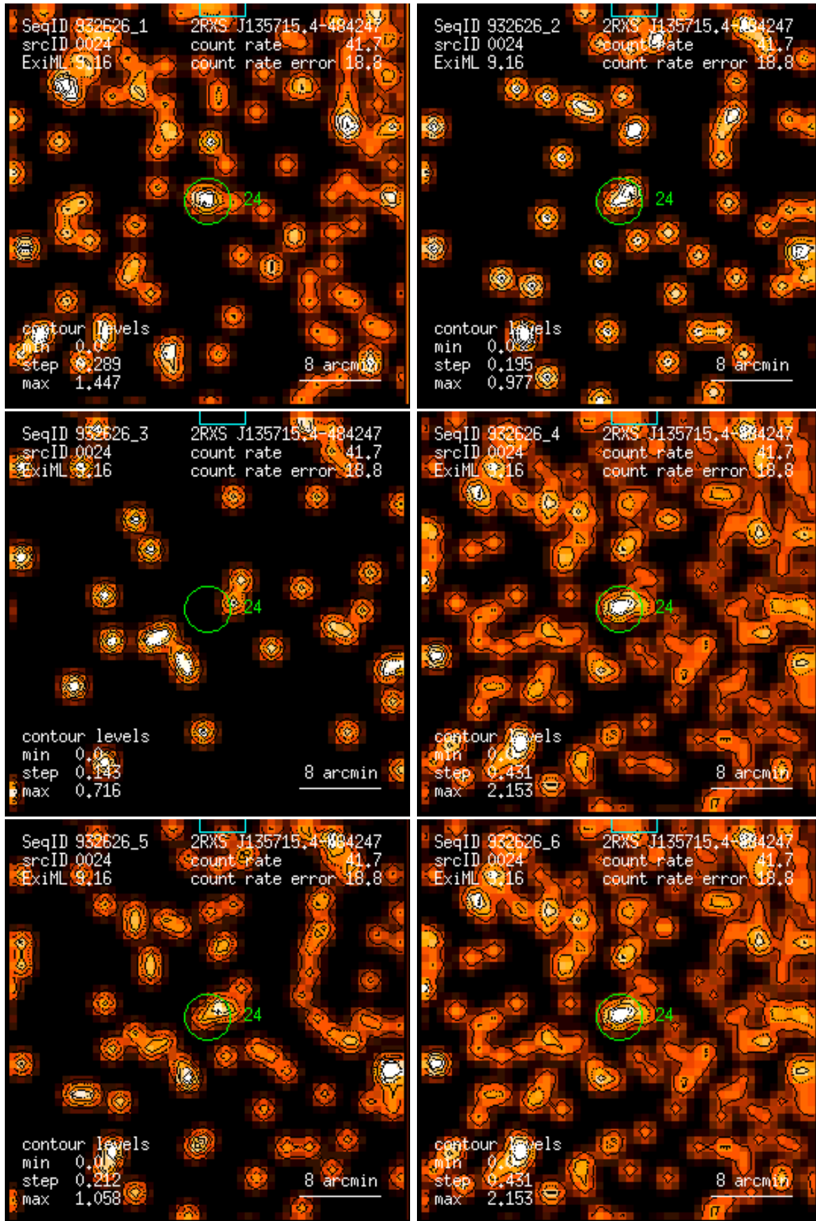
Figure 24: RASS 932626: detection 0024: band rate images, Gaussian filter: (1) PSPC channels 11 – 41, (2) 52 – 90, (3) 91 – 201, (4) 11 – 235, (5) 52 – 201, (6) 11 – 201. Broad band rates in counts/ks. Band rate contour levels in counts/ks/arcmin 2 .
