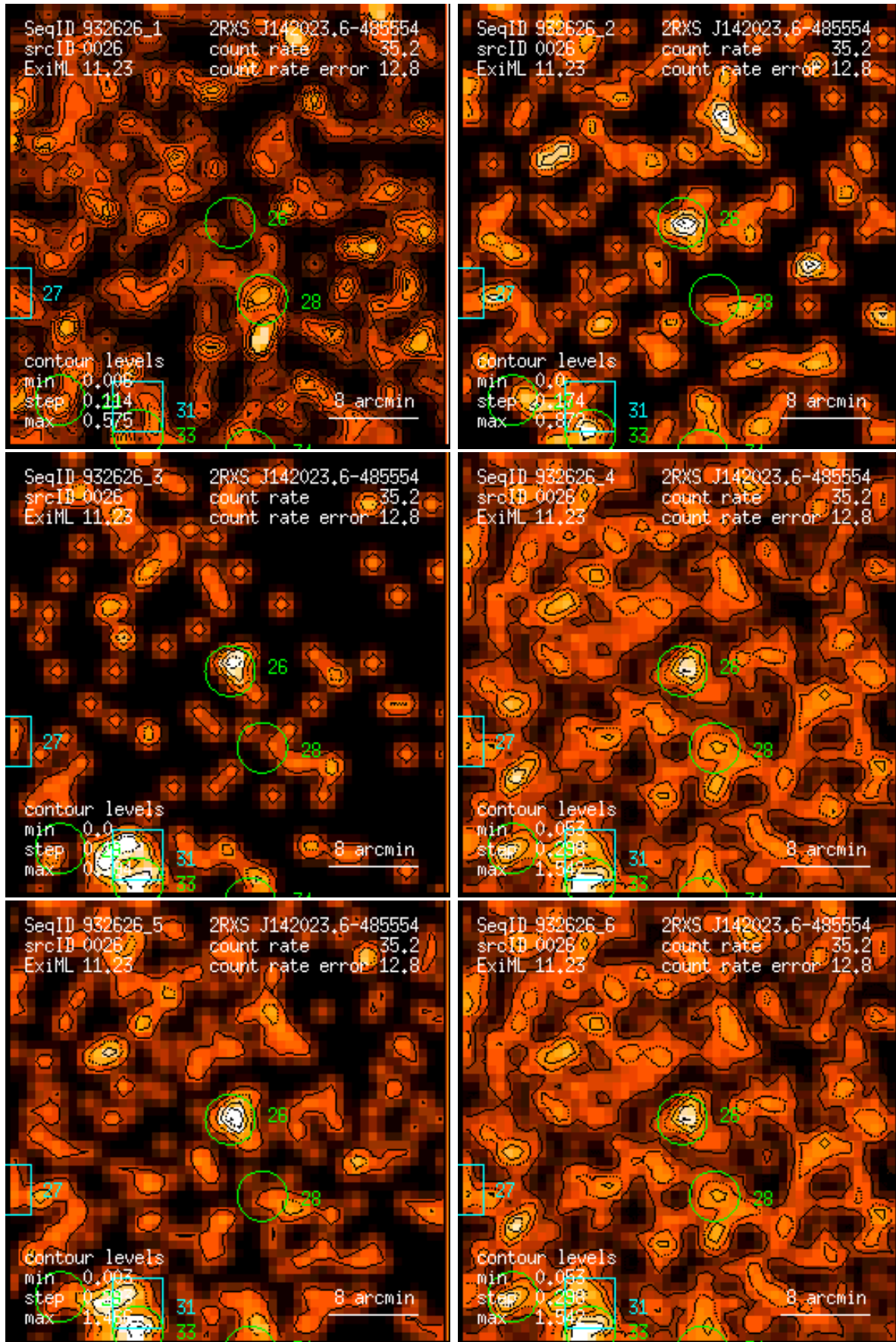
Figure 26: RASS 932626: detection 0026: band rate images, Gaussian filter: (1) PSPC channels 11 – 41, (2) 52 – 90, (3) 91 – 201, (4) 11 – 235, (5) 52 – 201, (6) 11 – 201. Broad band rates in counts/ks. Band rate contour levels in counts/ks/arcmin 2 .
