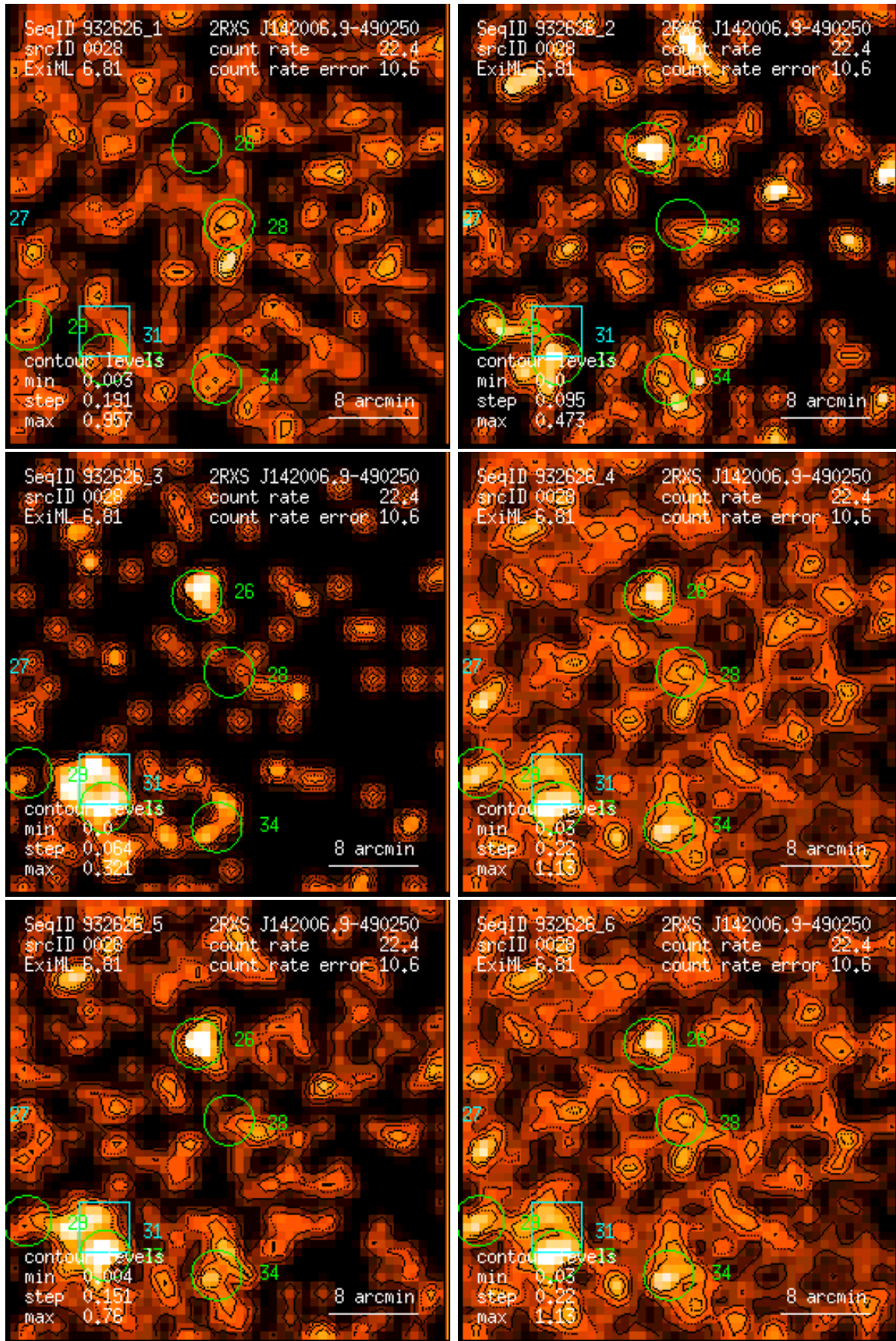
Figure 28: RASS 932626: detection 0028: band rate images, Gaussian filter: (1) PSPC channels 11 – 41, (2) 52 – 90, (3) 91 – 201, (4) 11 – 235, (5) 52 – 201, (6) 11 – 201. Broad band rates in counts/ks. Band rate contour levels in counts/ks/arcmin 2 .
