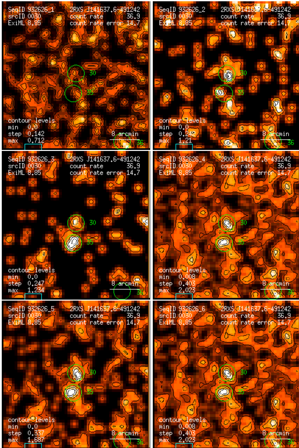
Figure 30: RASS 932626: detection 0030: band rate images, Gaussian filter: (1) PSPC channels 11 – 41, (2) 52 – 90, (3) 91 – 201, (4) 11 – 235, (5) 52 – 201, (6) 11 – 201. Broad band rates in counts/ks. Band rate contour levels in counts/ks/arcmin 2 .
