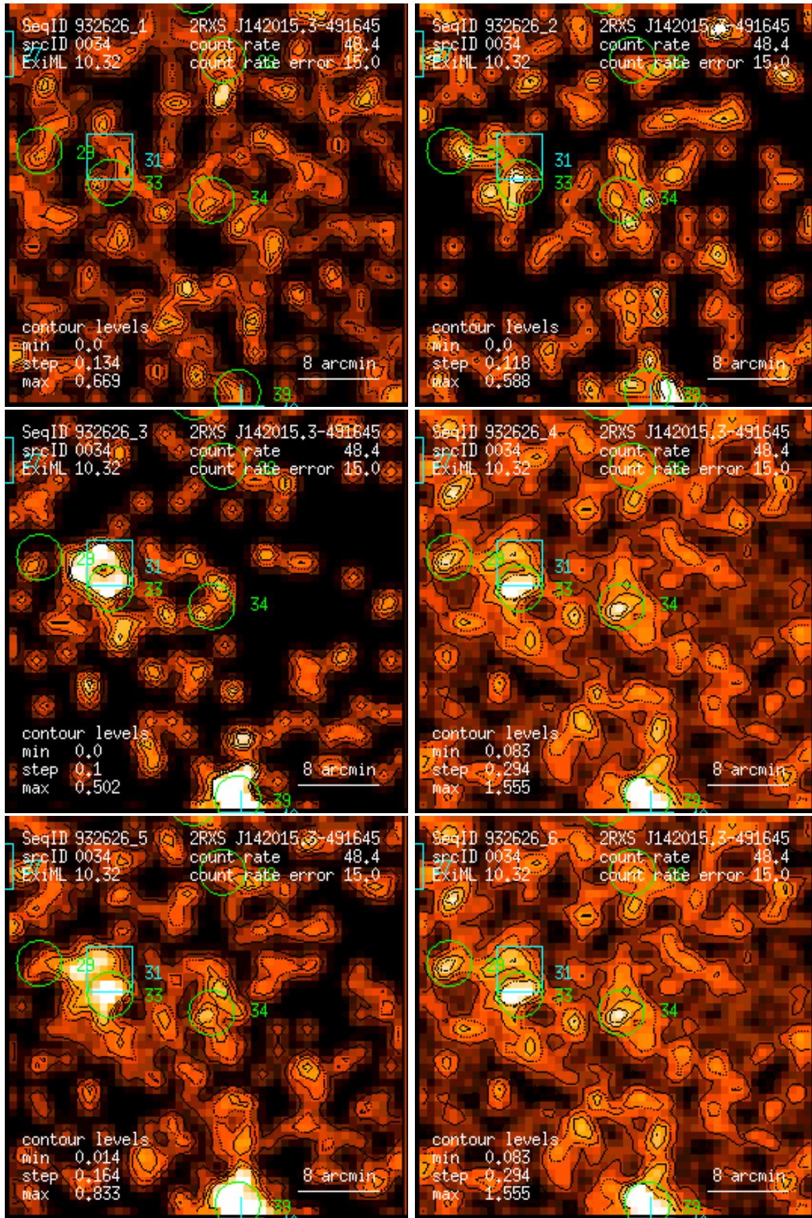
Figure 34: RASS 932626: detection 0034: band rate images, Gaussian filter: (1) PSPC channels 11 – 41, (2) 52 – 90, (3) 91 – 201, (4) 11 – 235, (5) 52 – 201, (6) 11 – 201. Broad band rates in counts/ks. Band rate contour levels in counts/ks/arcmin 2 .
