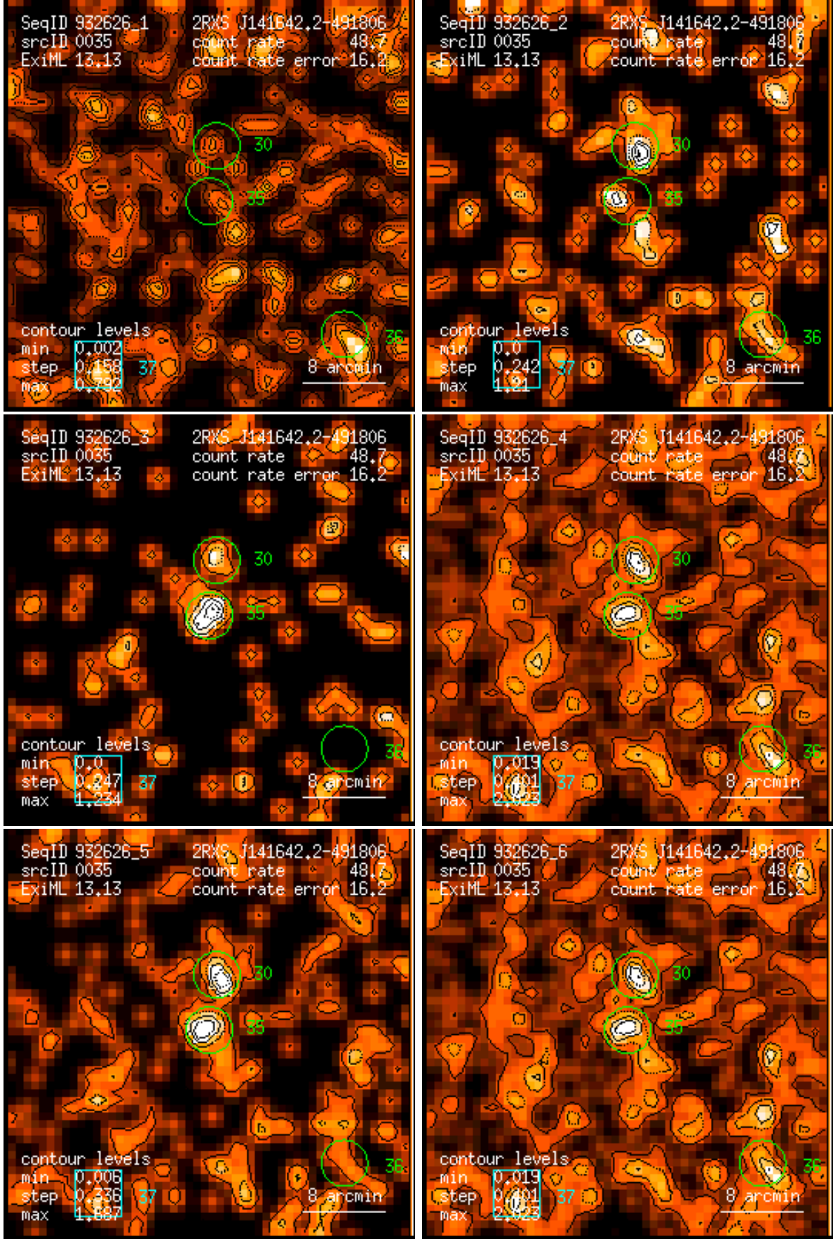
Figure 35: RASS 932626: detection 0035: band rate images, Gaussian filter: (1) PSPC channels 11 – 41, (2) 52 – 90, (3) 91 – 201, (4) 11 – 235, (5) 52 – 201, (6) 11 – 201. Broad band rates in counts/ks. Band rate contour levels in counts/ks/arcmin 2 .
