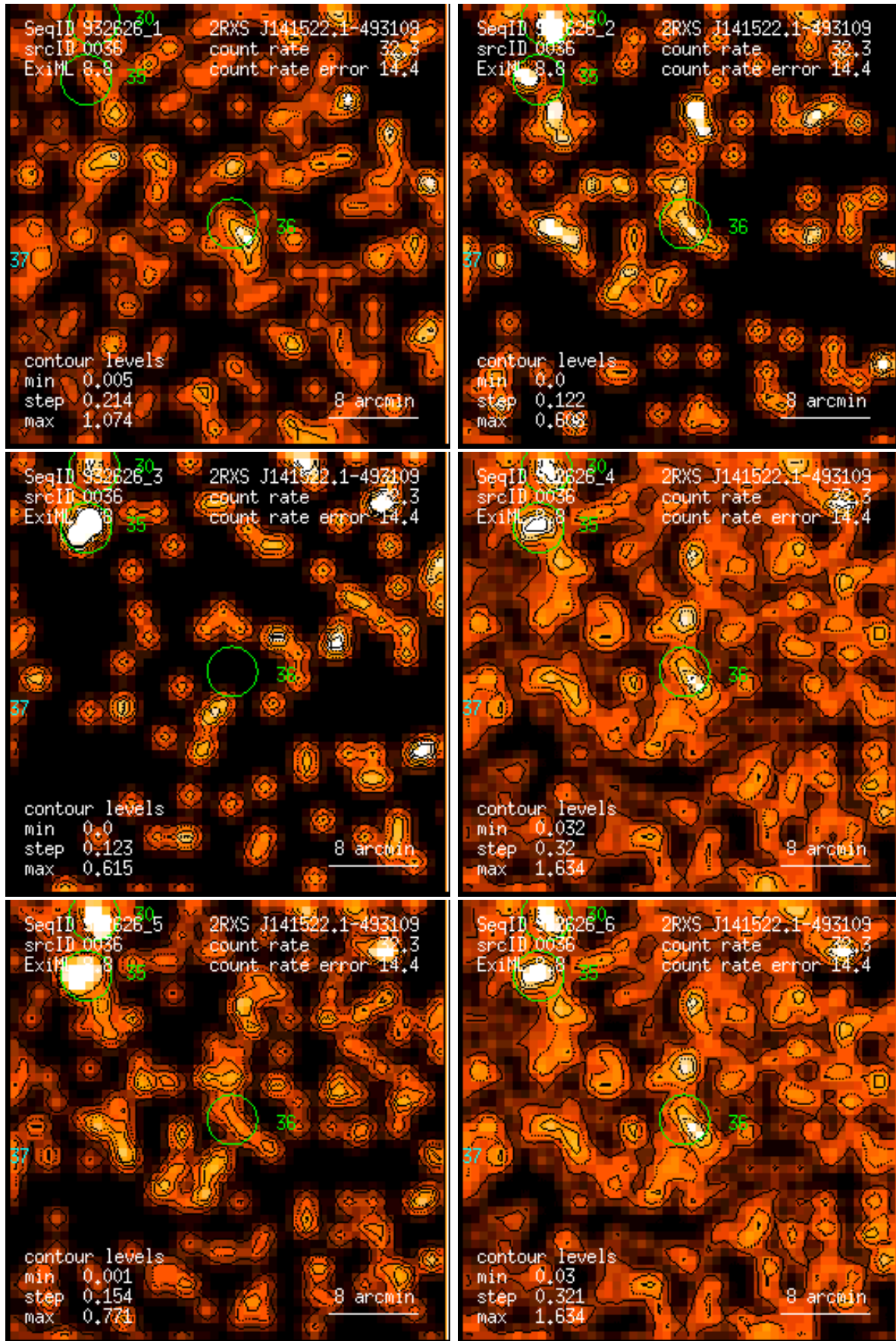
Figure 36: RASS 932626: detection 0036: band rate images, Gaussian filter: (1) PSPC channels 11 – 41, (2) 52 – 90, (3) 91 – 201, (4) 11 – 235, (5) 52 – 201, (6) 11 – 201. Broad band rates in counts/ks. Band rate contour levels in counts/ks/arcmin 2 .
