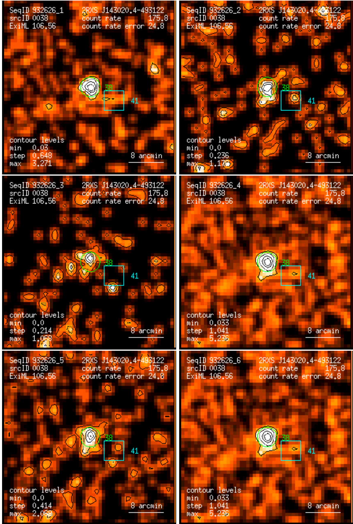
Figure 38: RASS 932626: detection 0038: band rate images, Gaussian filter: (1) PSPC channels 11 – 41, (2) 52 – 90, (3) 91 – 201, (4) 11 – 235, (5) 52 – 201, (6) 11 – 201. Broad band rates in counts/ks. Band rate contour levels in counts/ks/arcmin 2 .
