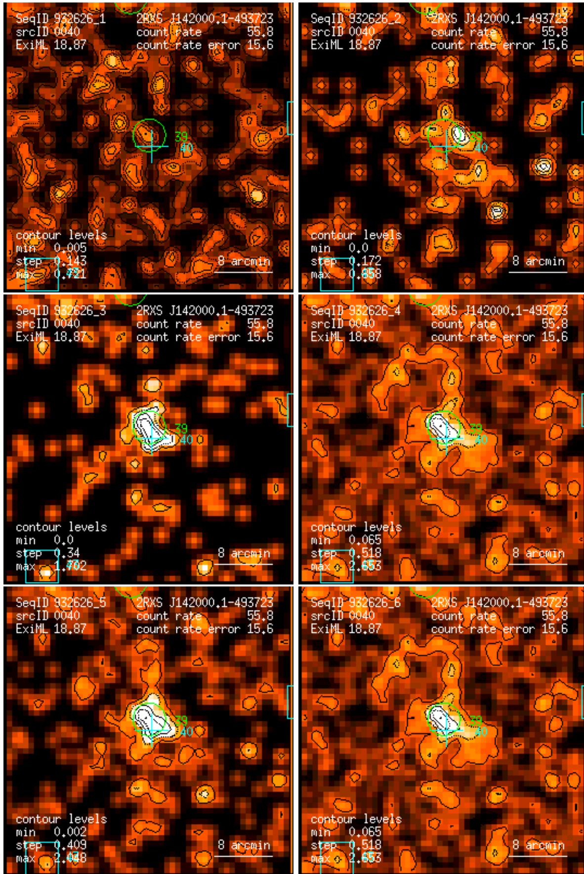
Figure 40: RASS 932626: detection 0040: band rate images, Gaussian filter: (1) PSPC channels 11 – 41, (2) 52 – 90, (3) 91 – 201, (4) 11 – 235, (5) 52 – 201, (6) 11 – 201. Broad band rates in counts/ks. Band rate contour levels in counts/ks/arcmin 2 .
