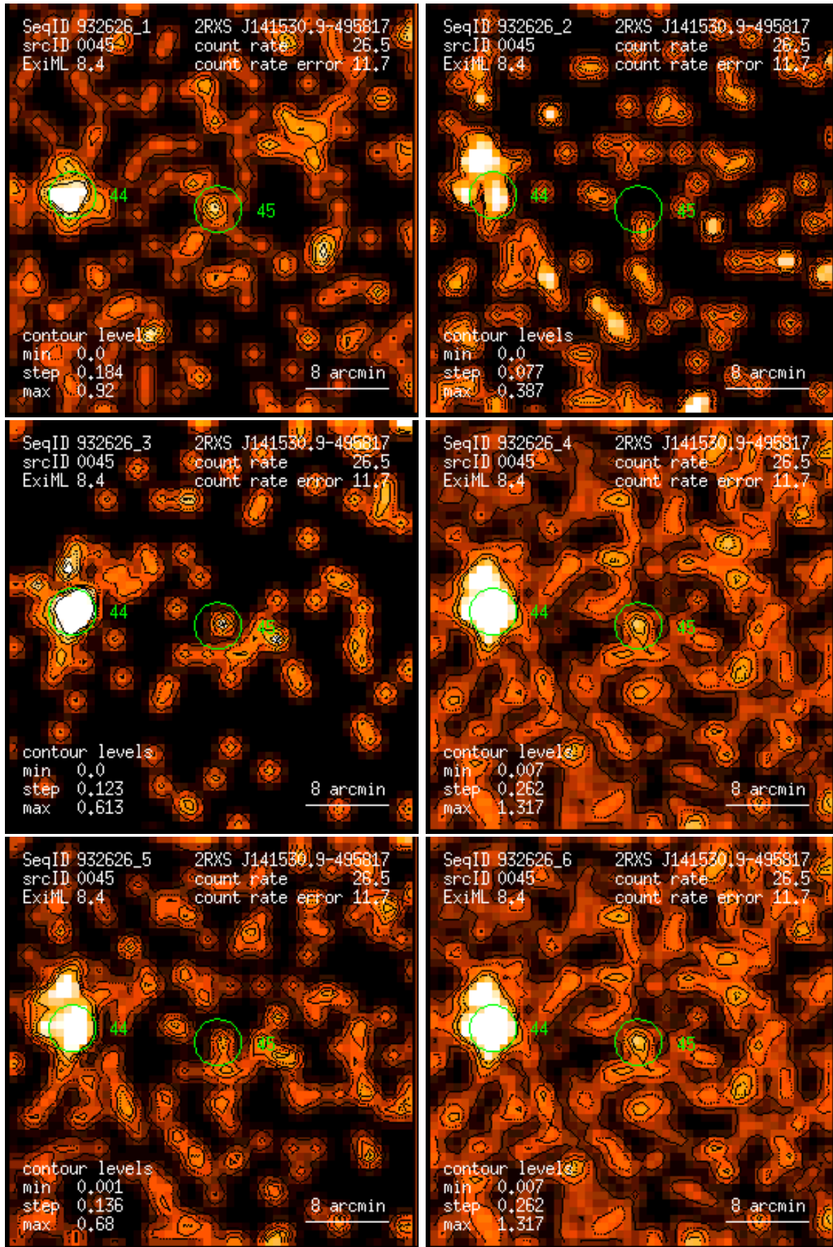
Figure 45: RASS 932626: detection 0045: band rate images, Gaussian filter: (1) PSPC channels 11 – 41, (2) 52 – 90, (3) 91 – 201, (4) 11 – 235, (5) 52 – 201, (6) 11 – 201. Broad band rates in counts/ks. Band rate contour levels in counts/ks/arcmin 2 .
