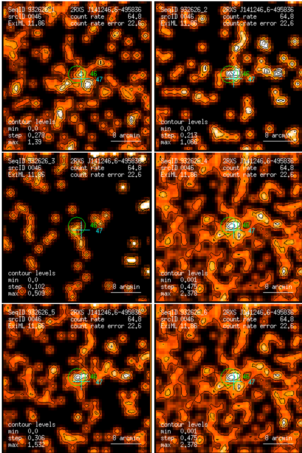
Figure 46: RASS 932626: detection 0046: band rate images, Gaussian filter: (1) PSPC channels 11 – 41, (2) 52 – 90, (3) 91 – 201, (4) 11 – 235, (5) 52 – 201, (6) 11 – 201. Broad band rates in counts/ks. Band rate contour levels in counts/ks/arcmin 2 .
