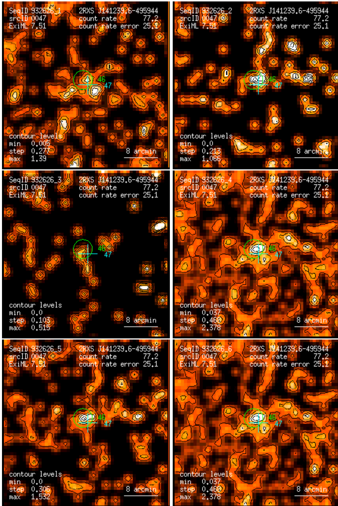
Figure 47: RASS 932626: detection 0047: band rate images, Gaussian filter: (1) PSPC channels 11 – 41, (2) 52 – 90, (3) 91 – 201, (4) 11 – 235, (5) 52 – 201, (6) 11 – 201. Broad band rates in counts/ks. Band rate contour levels in counts/ks/arcmin 2 .
