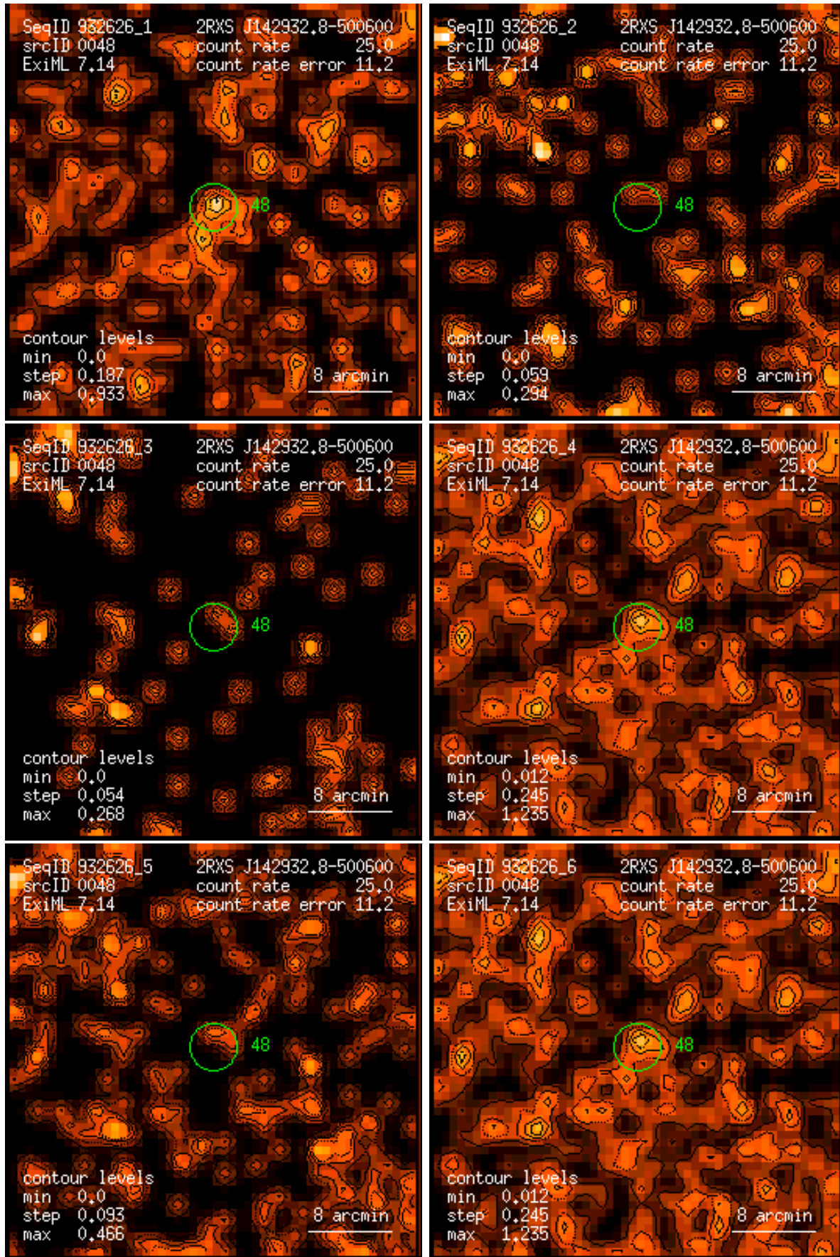
Figure 48: RASS 932626: detection 0048: band rate images, Gaussian filter: (1) PSPC channels 11 – 41, (2) 52 – 90, (3) 91 – 201, (4) 11 – 235, (5) 52 – 201, (6) 11 – 201. Broad band rates in counts/ks. Band rate contour levels in counts/ks/arcmin 2 .
