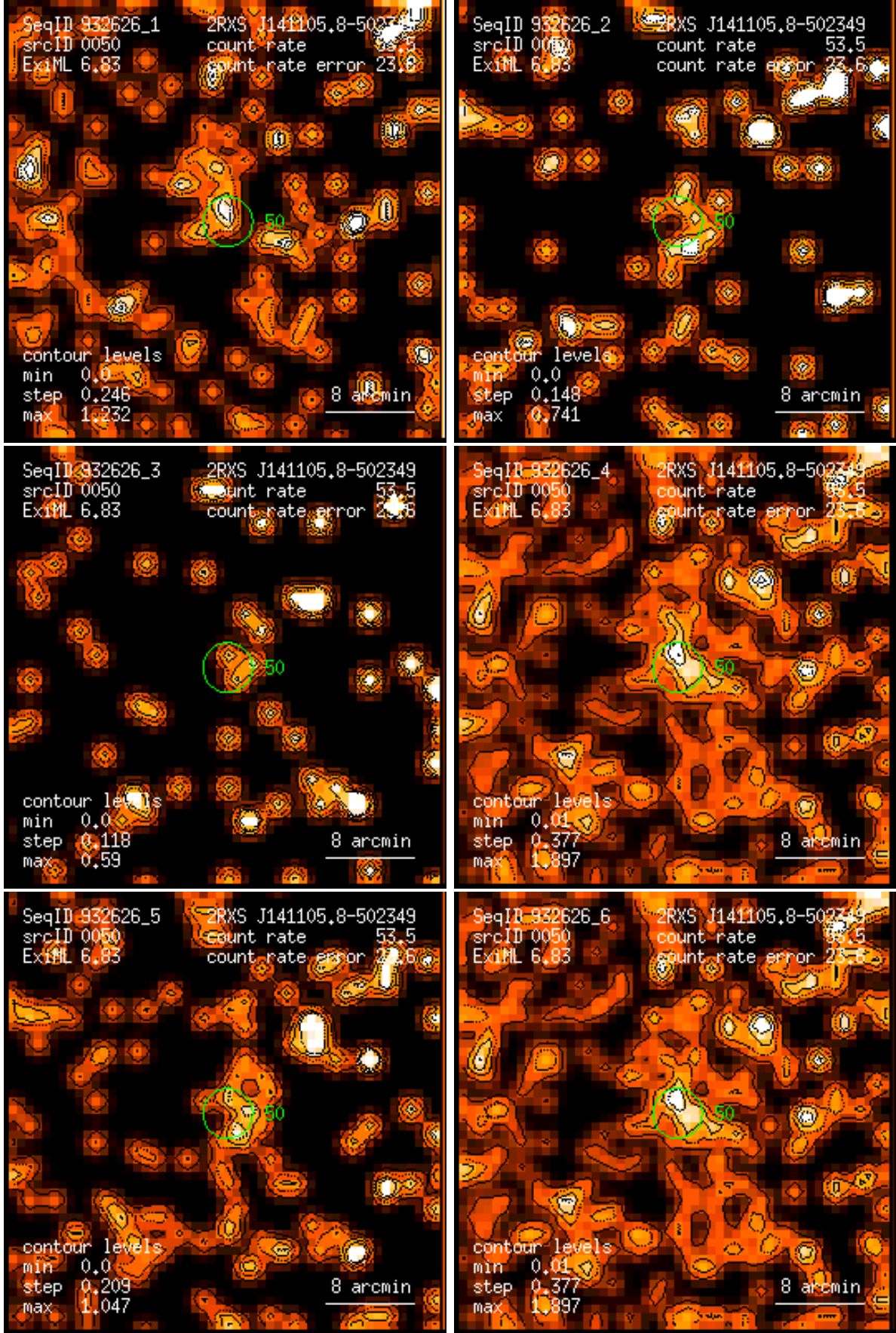
Figure 50: RASS 932626: detection 0050: band rate images, Gaussian filter: (1) PSPC channels 11 – 41, (2) 52 – 90, (3) 91 – 201, (4) 11 – 235, (5) 52 – 201, (6) 11 – 201. Broad band rates in counts/ks. Band rate contour levels in counts/ks/arcmin 2 .
