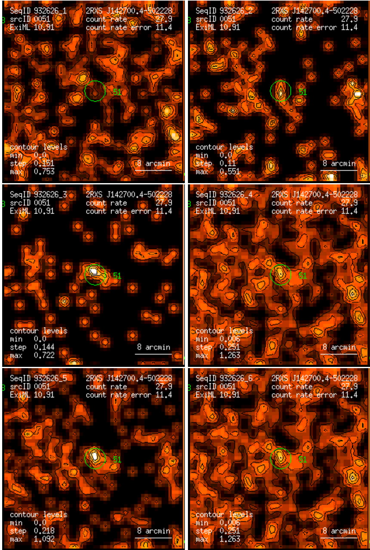
Figure 51: RASS 932626: detection 0051: band rate images, Gaussian filter: (1) PSPC channels 11 – 41, (2) 52 – 90, (3) 91 – 201, (4) 11 – 235, (5) 52 – 201, (6) 11 – 201. Broad band rates in counts/ks. Band rate contour levels in counts/ks/arcmin 2 .
