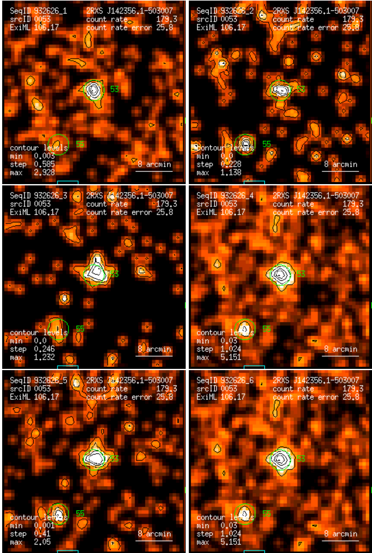
Figure 53: RASS 932626: detection 0053: band rate images, Gaussian filter: (1) PSPC channels 11 – 41, (2) 52 – 90, (3) 91 – 201, (4) 11 – 235, (5) 52 – 201, (6) 11 – 201. Broad band rates in counts/ks. Band rate contour levels in counts/ks/arcmin 2 .
