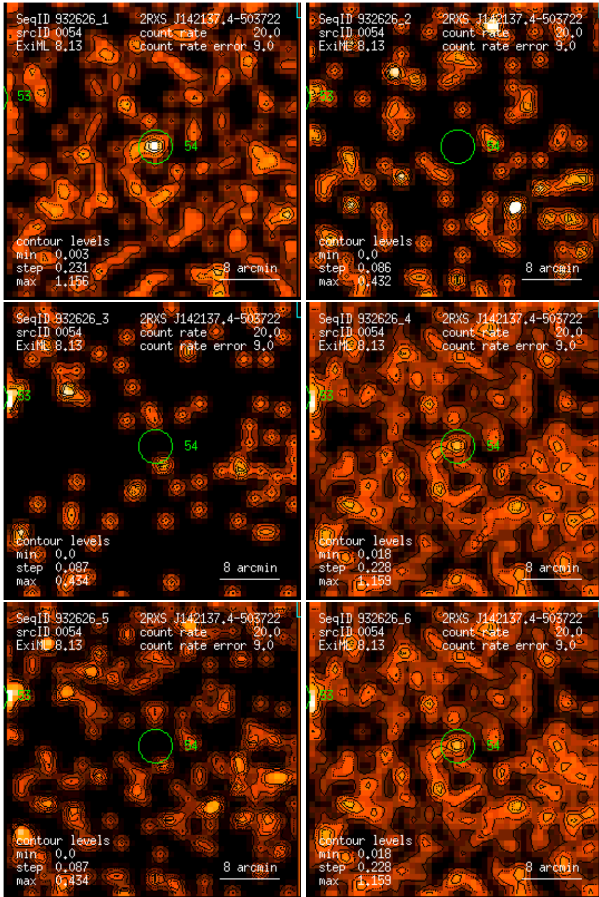
Figure 54: RASS 932626: detection 0054: band rate images, Gaussian filter: (1) PSPC channels 11 – 41, (2) 52 – 90, (3) 91 – 201, (4) 11 – 235, (5) 52 – 201, (6) 11 – 201. Broad band rates in counts/ks. Band rate contour levels in counts/ks/arcmin 2 .
