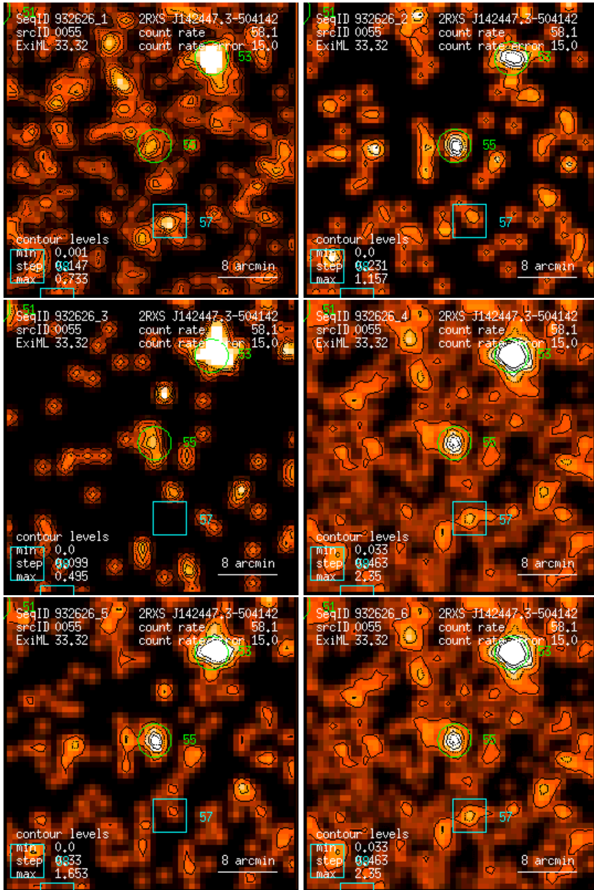
Figure 55: RASS 932626: detection 0055: band rate images, Gaussian filter: (1) PSPC channels 11 – 41, (2) 52 – 90, (3) 91 – 201, (4) 11 – 235, (5) 52 – 201, (6) 11 – 201. Broad band rates in counts/ks. Band rate contour levels in counts/ks/arcmin 2 .
