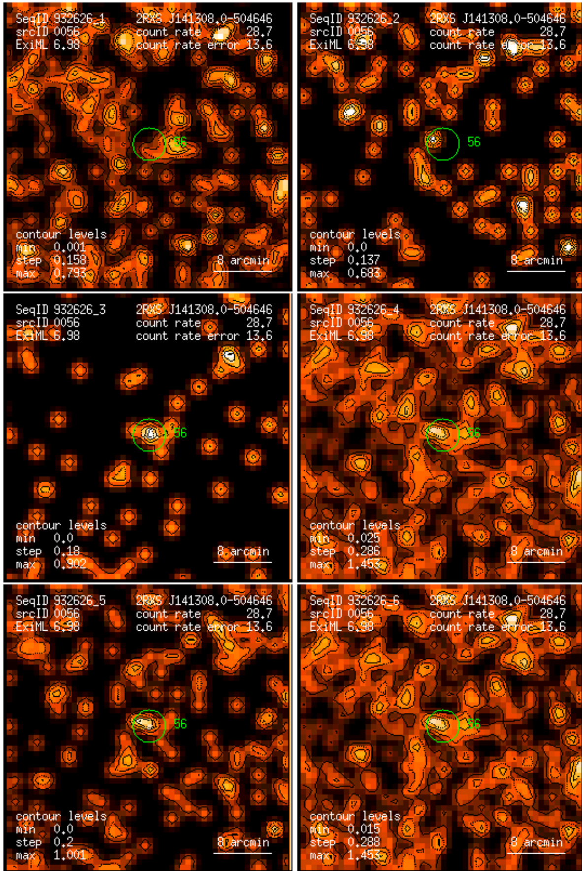
Figure 56: RASS 932626: detection 0056: band rate images, Gaussian filter: (1) PSPC channels 11 – 41, (2) 52 – 90, (3) 91 – 201, (4) 11 – 235, (5) 52 – 201, (6) 11 – 201. Broad band rates in counts/ks. Band rate contour levels in counts/ks/arcmin 2 .
