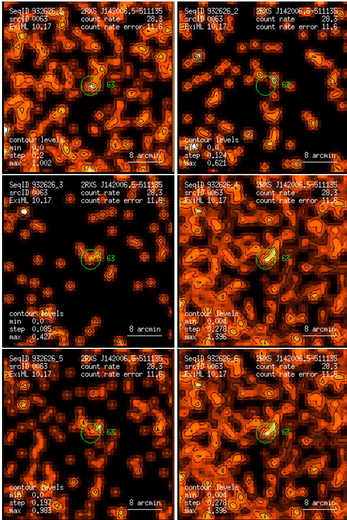
Figure 63: RASS 932626: detection 0063: band rate images, Gaussian filter: (1) PSPC channels 11 – 41, (2) 52 – 90, (3) 91 – 201, (4) 11 – 235, (5) 52 – 201, (6) 11 – 201. Broad band rates in counts/ks. Band rate contour levels in counts/ks/arcmin 2 .
