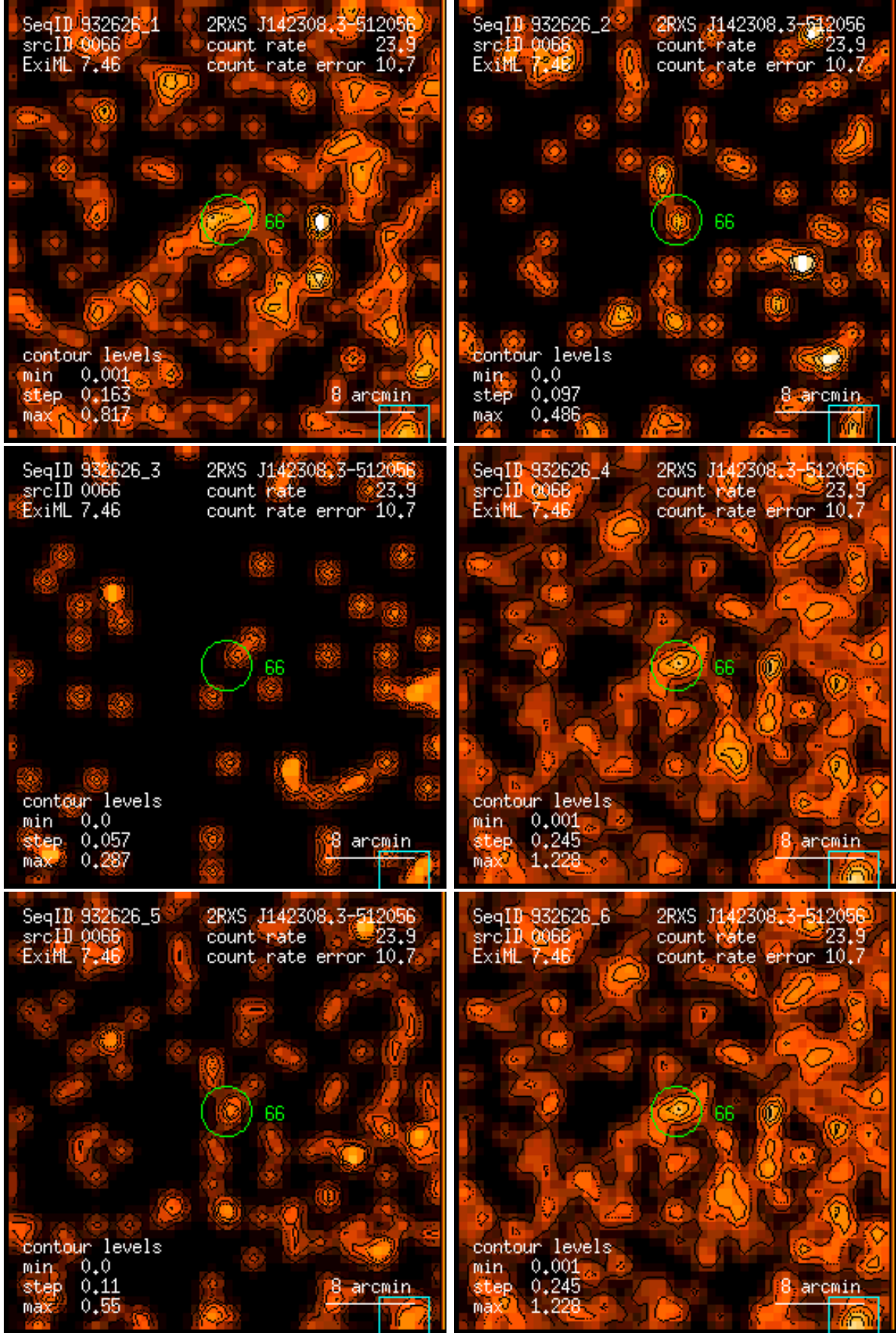
Figure 66: RASS 932626: detection 0066: band rate images, Gaussian filter: (1) PSPC channels 11 – 41, (2) 52 – 90, (3) 91 – 201, (4) 11 – 235, (5) 52 – 201, (6) 11 – 201. Broad band rates in counts/ks. Band rate contour levels in counts/ks/arcmin 2 .
