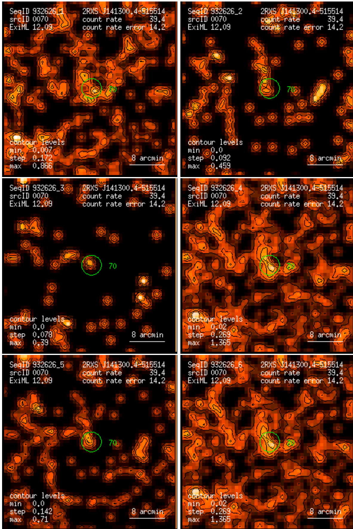
Figure 70: RASS 932626: detection 0070: band rate images, Gaussian filter: (1) PSPC channels 11 – 41, (2) 52 – 90, (3) 91 – 201, (4) 11 – 235, (5) 52 – 201, (6) 11 – 201. Broad band rates in counts/ks. Band rate contour levels in counts/ks/arcmin 2 .
