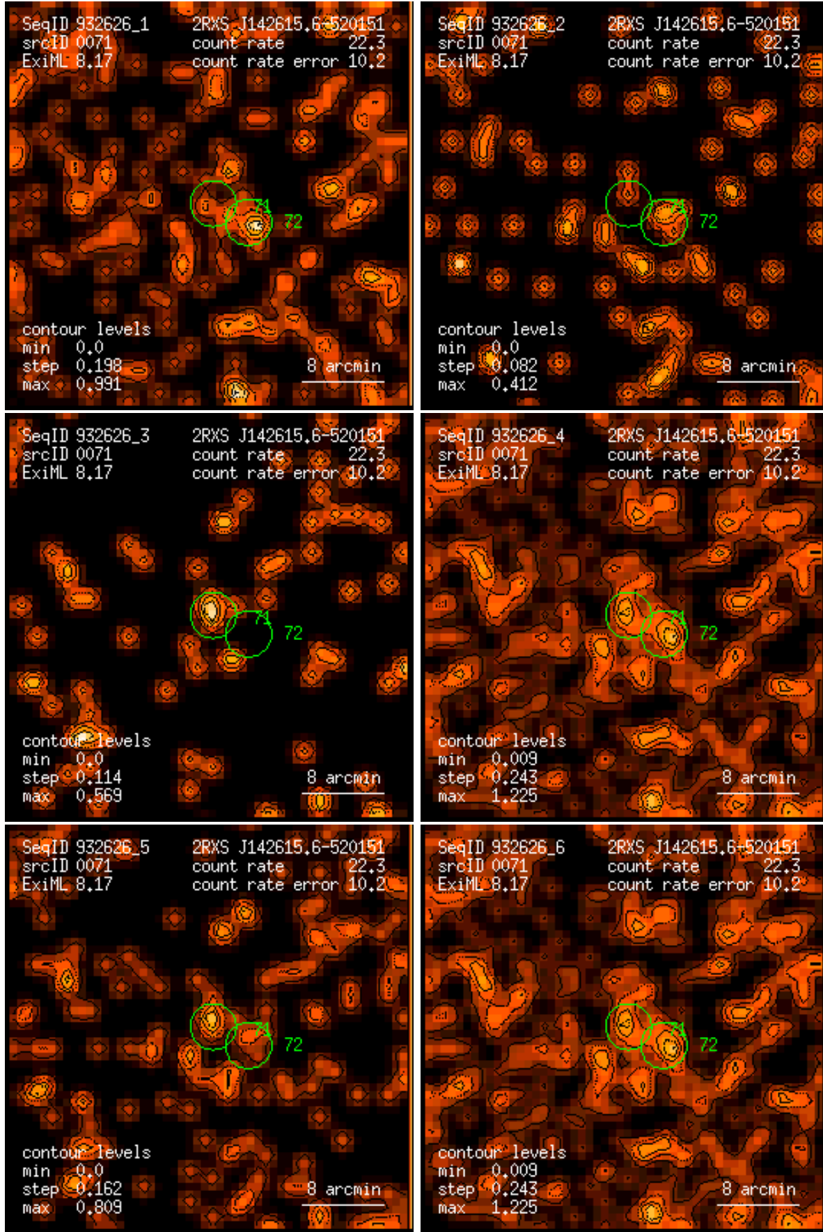
Figure 71: RASS 932626: detection 0071: band rate images, Gaussian filter: (1) PSPC channels 11 – 41, (2) 52 – 90, (3) 91 – 201, (4) 11 – 235, (5) 52 – 201, (6) 11 – 201. Broad band rates in counts/ks. Band rate contour levels in counts/ks/arcmin 2 .
