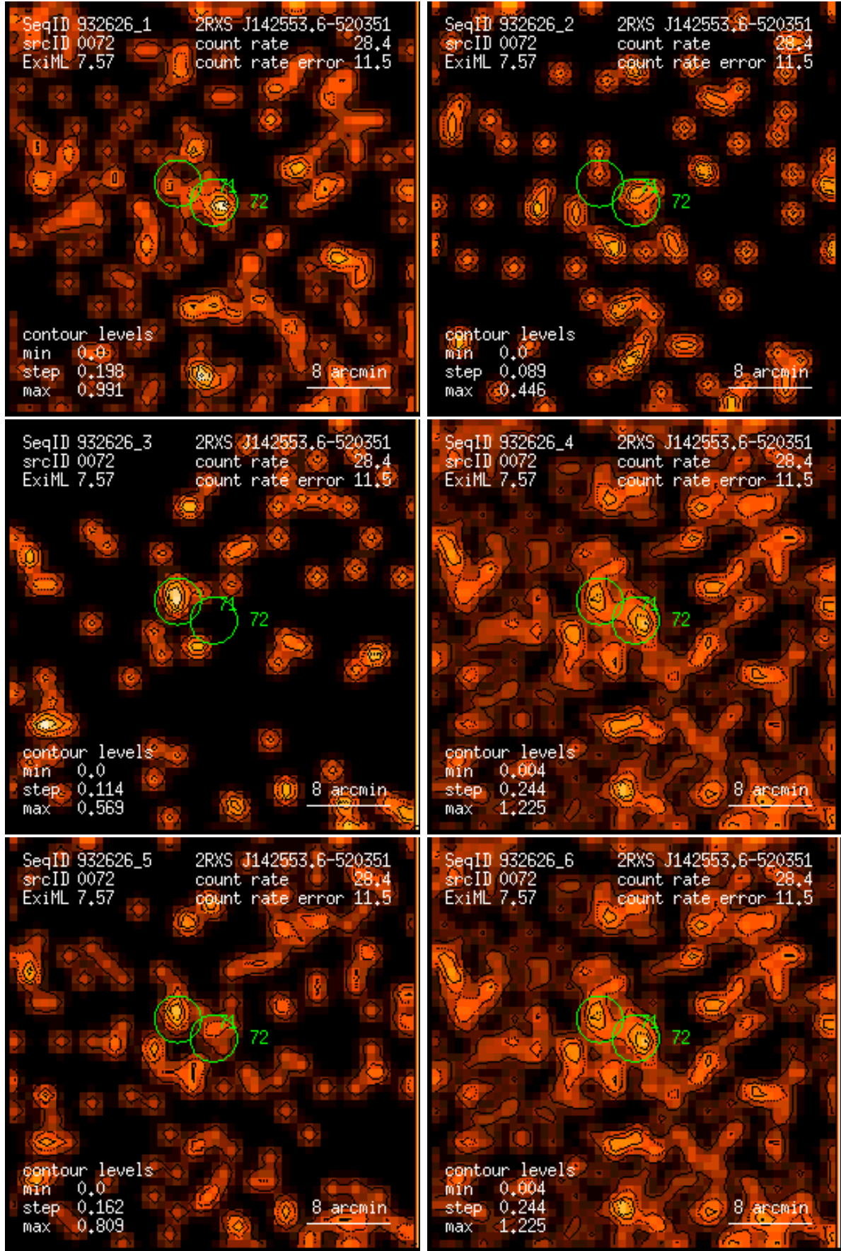
Figure 72: RASS 932626: detection 0072: band rate images, Gaussian filter: (1) PSPC channels 11 – 41, (2) 52 – 90, (3) 91 – 201, (4) 11 – 235, (5) 52 – 201, (6) 11 – 201. Broad band rates in counts/ks. Band rate contour levels in counts/ks/arcmin 2 .
