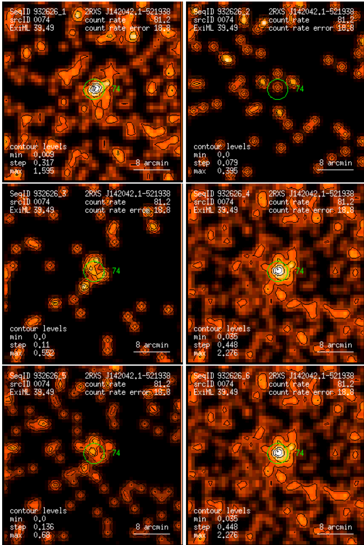
Figure 74: RASS 932626: detection 0074: band rate images, Gaussian filter: (1) PSPC channels 11 – 41, (2) 52 – 90, (3) 91 – 201, (4) 11 – 235, (5) 52 – 201, (6) 11 – 201. Broad band rates in counts/ks. Band rate contour levels in counts/ks/arcmin 2 .
