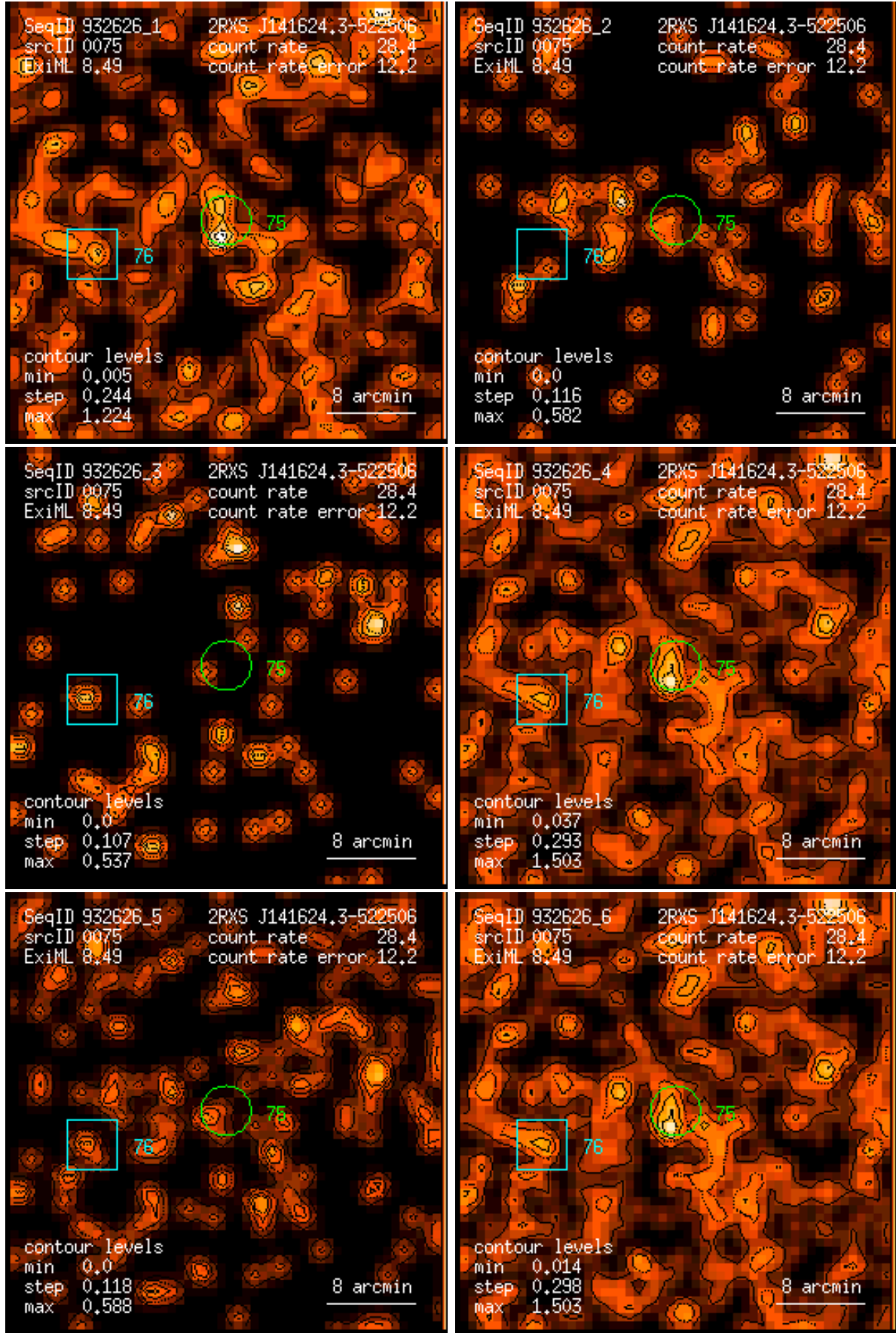
Figure 75: RASS 932626: detection 0075: band rate images, Gaussian filter: (1) PSPC channels 11 – 41, (2) 52 – 90, (3) 91 – 201, (4) 11 – 235, (5) 52 – 201, (6) 11 – 201. Broad band rates in counts/ks. Band rate contour levels in counts/ks/arcmin 2 .
