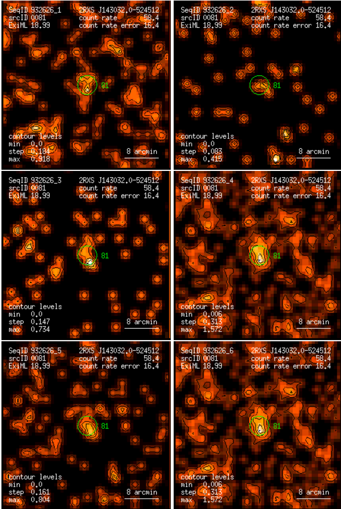
Figure 81: RASS 932626: detection 0081: band rate images, Gaussian filter: (1) PSPC channels 11 – 41, (2) 52 – 90, (3) 91 – 201, (4) 11 – 235, (5) 52 – 201, (6) 11 – 201. Broad band rates in counts/ks. Band rate contour levels in counts/ks/arcmin 2 .
