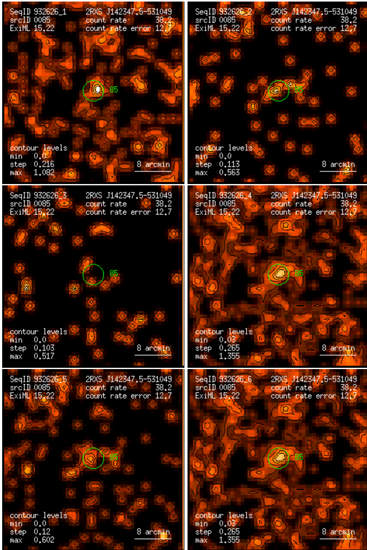
Figure 85: RASS 932626: detection 0085: band rate images, Gaussian filter: (1) PSPC channels 11 – 41, (2) 52 – 90, (3) 91 – 201, (4) 11 – 235, (5) 52 – 201, (6) 11 – 201. Broad band rates in counts/ks. Band rate contour levels in counts/ks/arcmin 2 .
