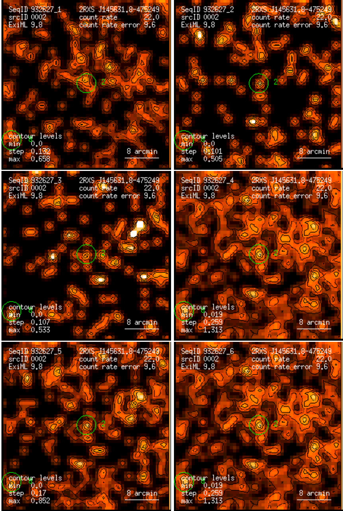
Figure 2: RASS 932627: detection 0002: band rate images, Gaussian filter: (1) PSPC channels 11 – 41, (2) 52 – 90, (3) 91 – 201, (4) 11 – 235, (5) 52 – 201, (6) 11 – 201. Broad band rates in counts/ks. Band rate contour levels in counts/ks/arcmin 2 .
